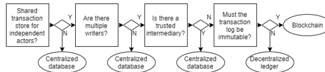
Fig. 1. TEAM decision tree for blockchain business cases.
